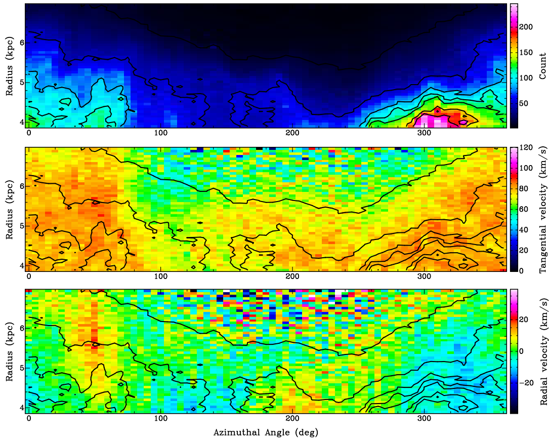
Fig. 21: Streaming motions across and along the eastern spiral arm of the LMC. The azimuth-radius diagrams show the stellar density (top panel), the tangential velocity (middle panel), and radial velocity (bottom panel). Contours represent the stellar density shown in the upper panel.
