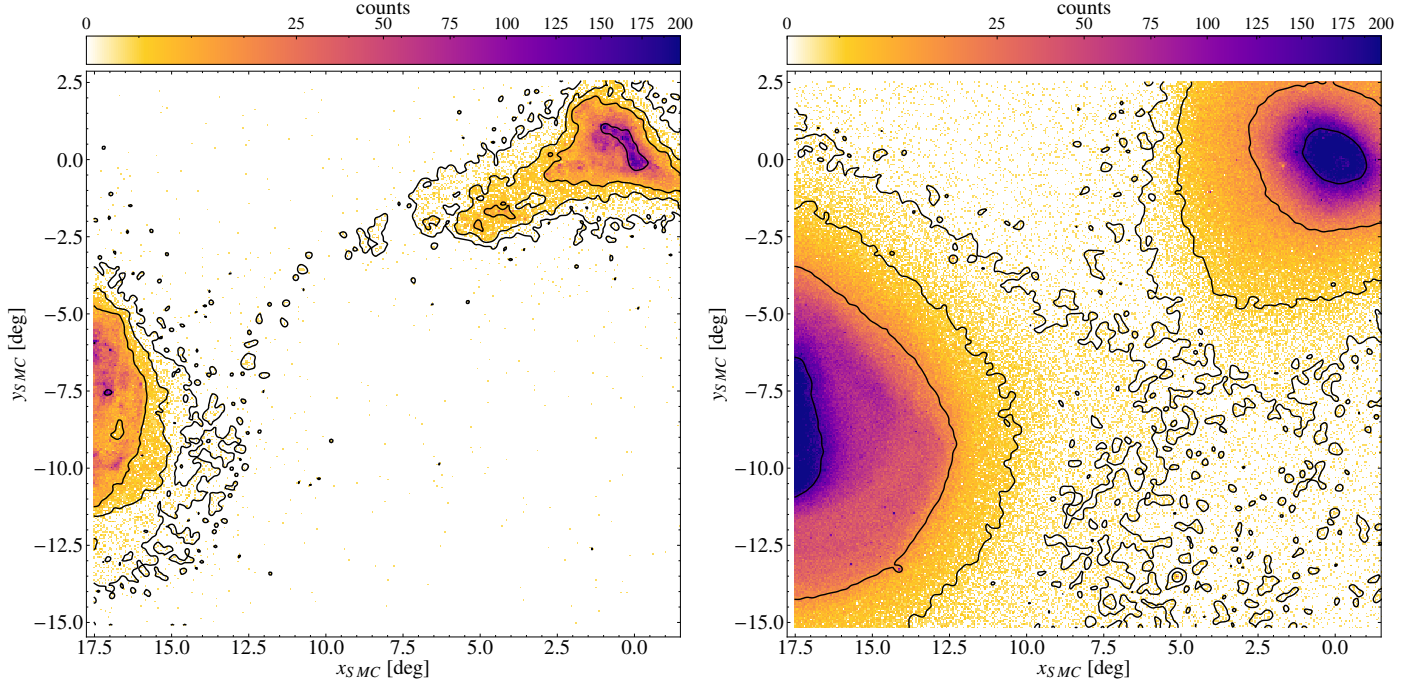
Fig. 15: Sky density plot for the Bridge region using the Young1 and Young2 evolutionary phases (left panel) and the RC evolutionary phase (right panel). The bin size is 0.06 deg in x and y . The colour bar is in log scale and the black contours are at the levels 0.1, 1, 5, and 70 (young evolutionary phases) and 0.25, 1.5, 15, and 165 (RC sample).
